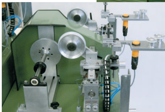
Fig.: winding solution with four winding stations
