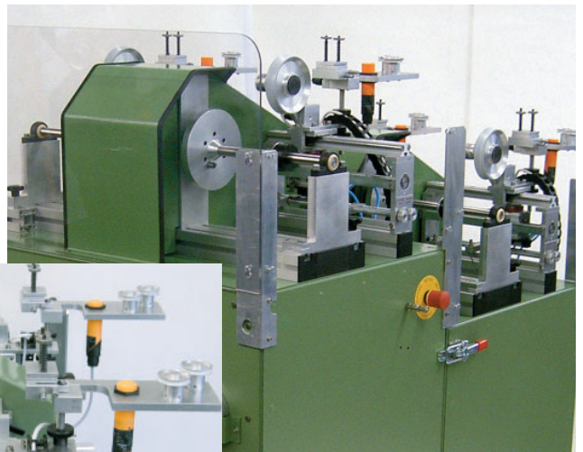
Fig.: winding solution with four winding stations
